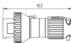
Plugue
