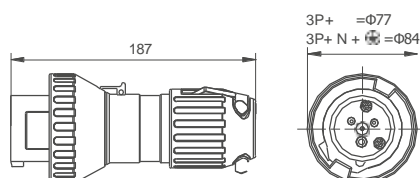
Plugue
